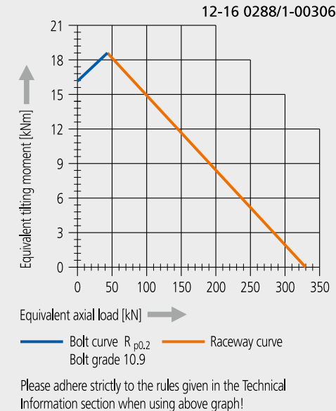
Limiting load diagram for "compressive" loads
