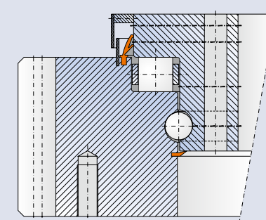
Cross section of a typical main Slewing Ring. This unit is a combination type with external toothing and a diameter of 4,800 mm (189 in).
