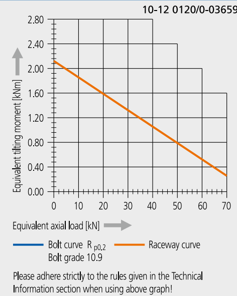
Limiting load diagram for "compressive" loads
