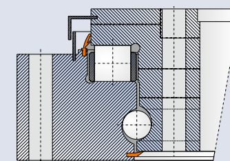
Bucket wheel excavators and stacker reclaimers use large diameter (over 5,000 mm – 196 in) Ball / Roller Combination Slewing Rings as main bearings.
