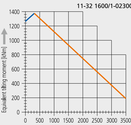
Limiting load diagram for "compressive" loads
