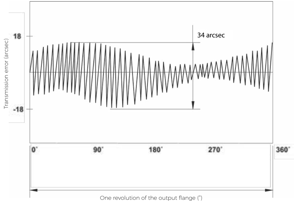
Fig. 3.9: Angular transmission error measurement
