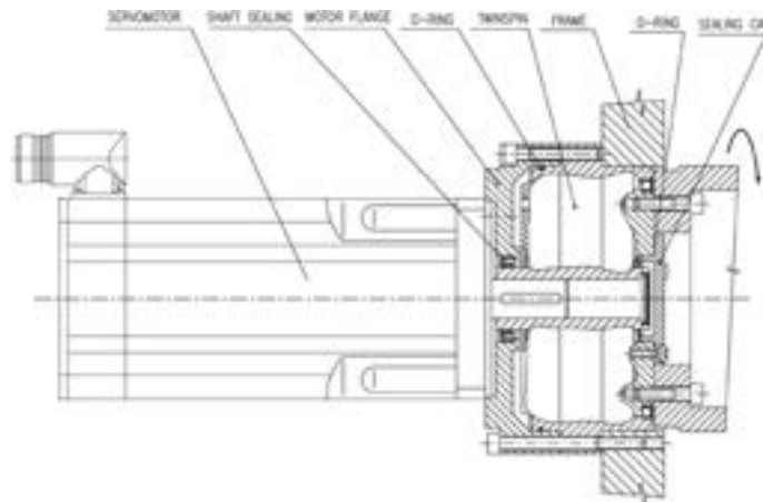
Fig. 5.2.1a: Direct connection of the reduction gear shaft with motor shaft
